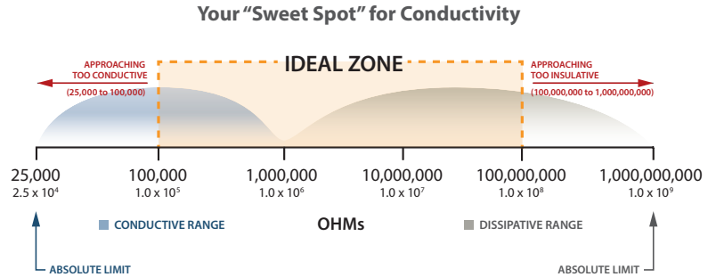
All Staticworx static-control flooring tests within the safe range (sweet spot) shown above.
