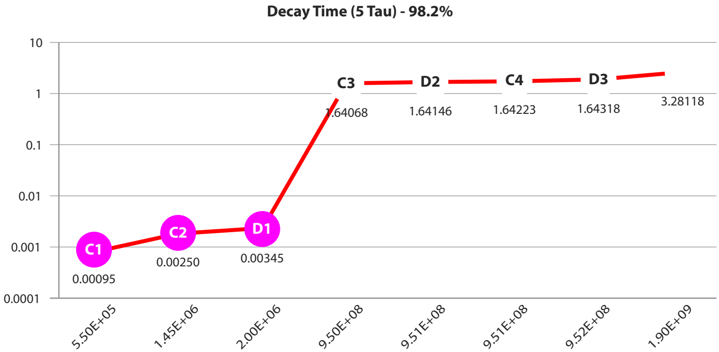
FIGURE 2: Decay Times for Flooring and Footwear Combinations (Logarithmic Scale)
